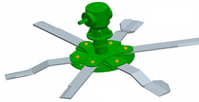
6-Blade High-Suction Mulching Rotor
