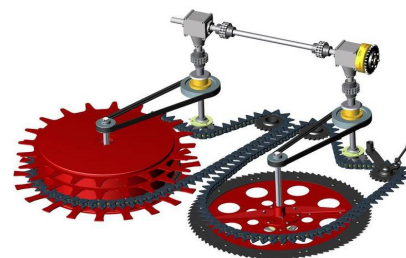
Power-Saving Even-Feed Drive
