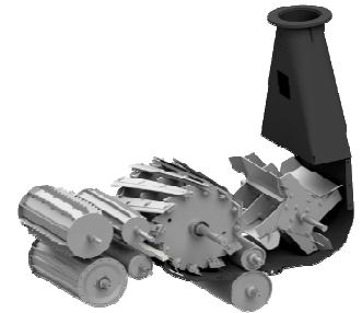
Straight-Thru Crop Flow
